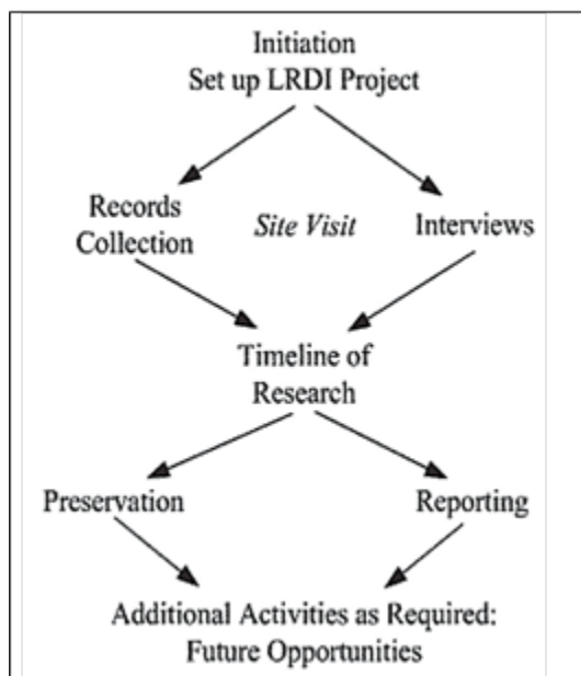
Figure 1. LRDI procedure.
