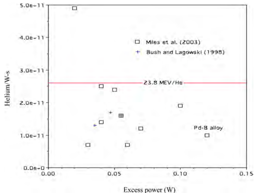
Figure 3. Comparison between several measurements of amount of helium released by the cathode divided by the energy measured as a function of excess power [37]. The expected ratio is shown by the horizontal line at 23.8 MeV/He. The cathode is palladium except in the one case when a Pd + B alloy is used, as indicated on the figure.
